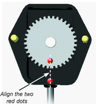
Fig B25 - Calibrating the rudder feedback unit
